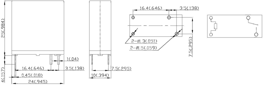
Internal Connections接线图 (Bottom View底视图)
